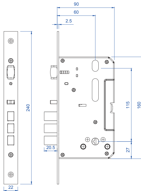
MAIN GATE MORTISE DG (400 | 402 | 404 | 405 | 406)
