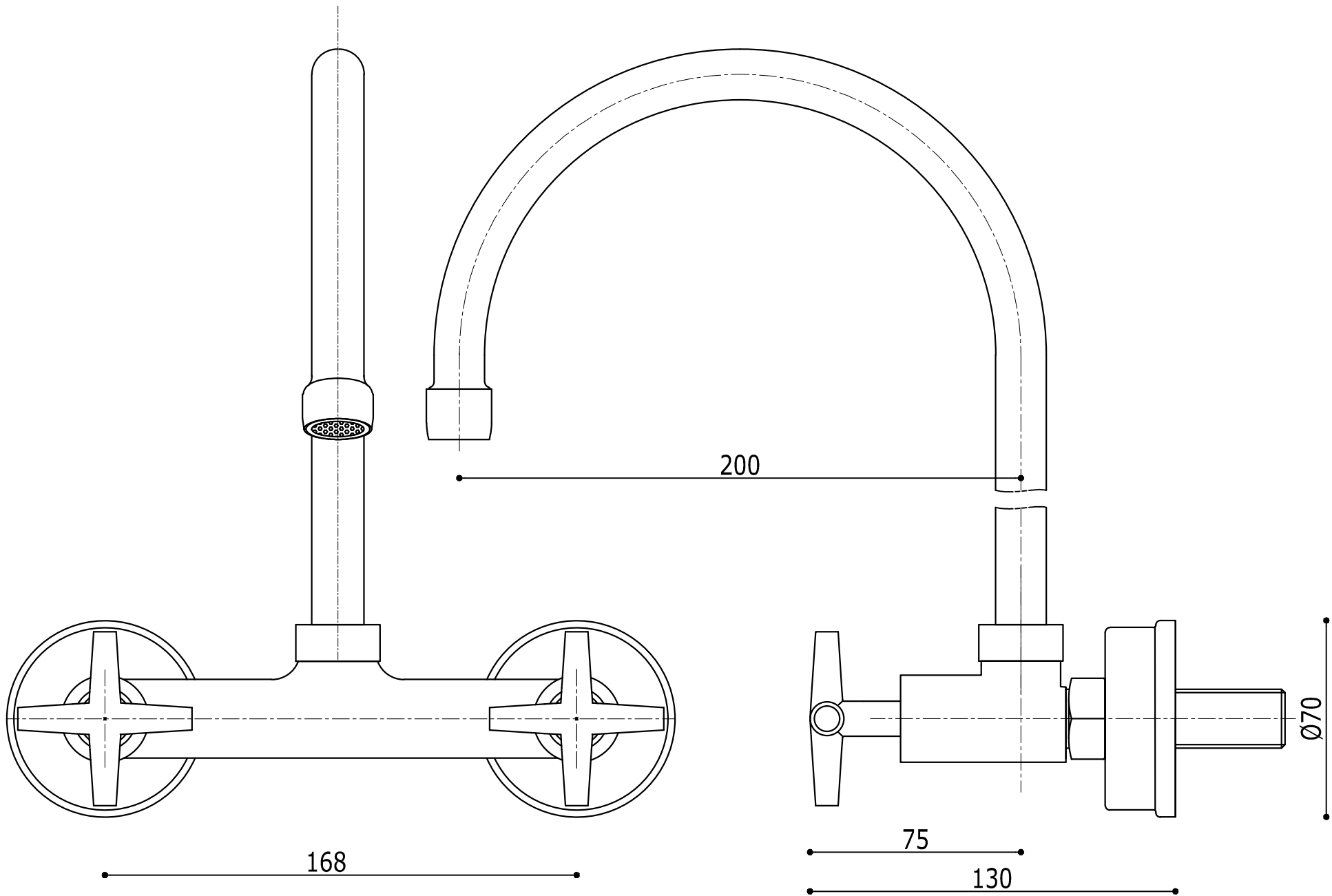
Sink Mixer Wall Mount
