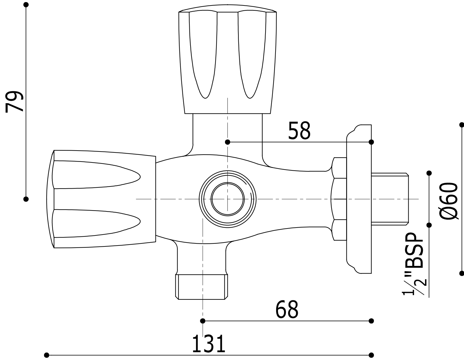
Two way Angular stop cock
